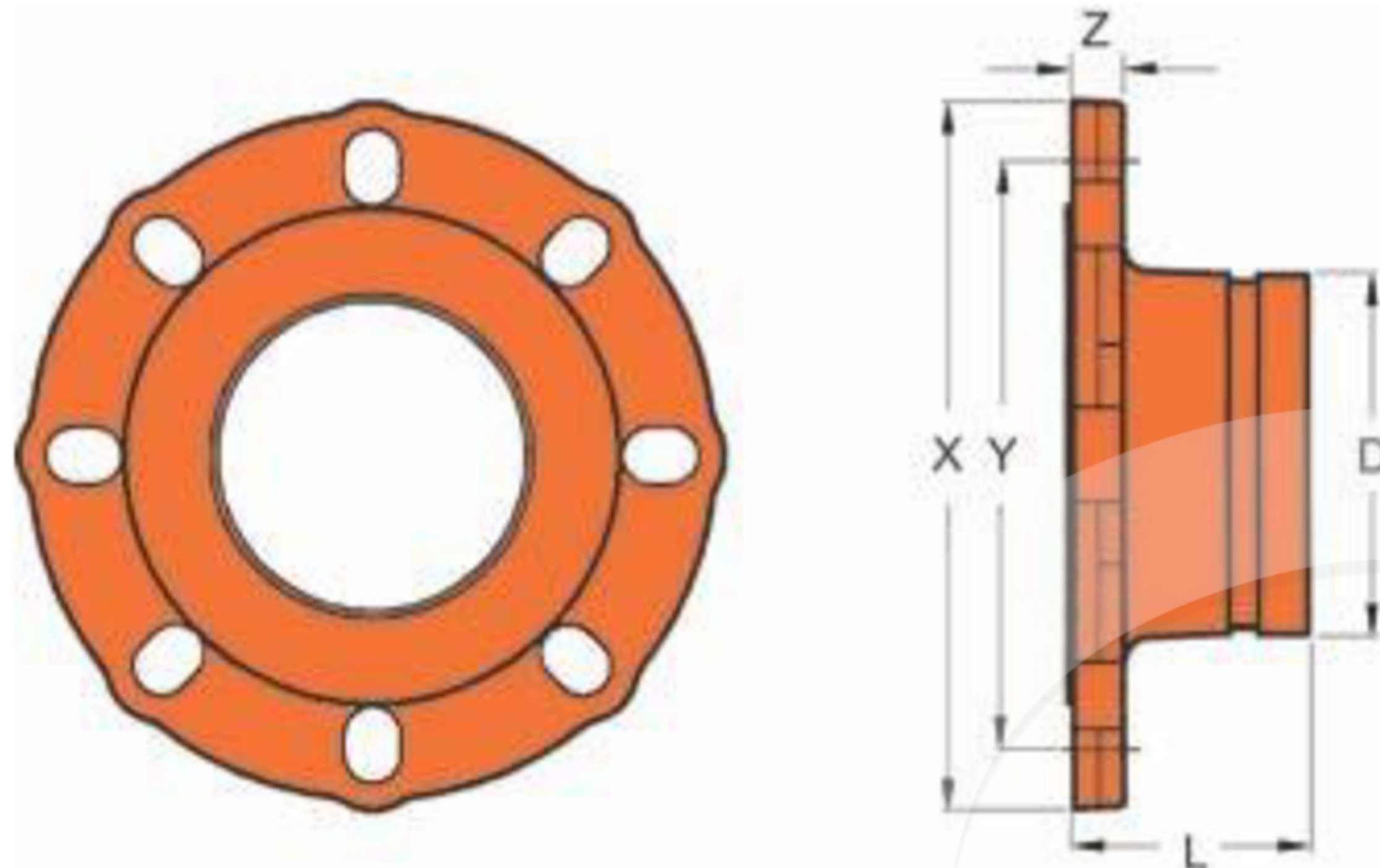
Model 7180 Universal Flange Adapter
